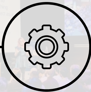
Data Engineering
